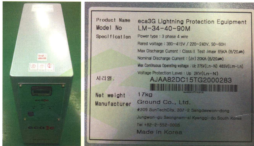
Photo. SG01 : Appearance of EUT(equipment under the test)
